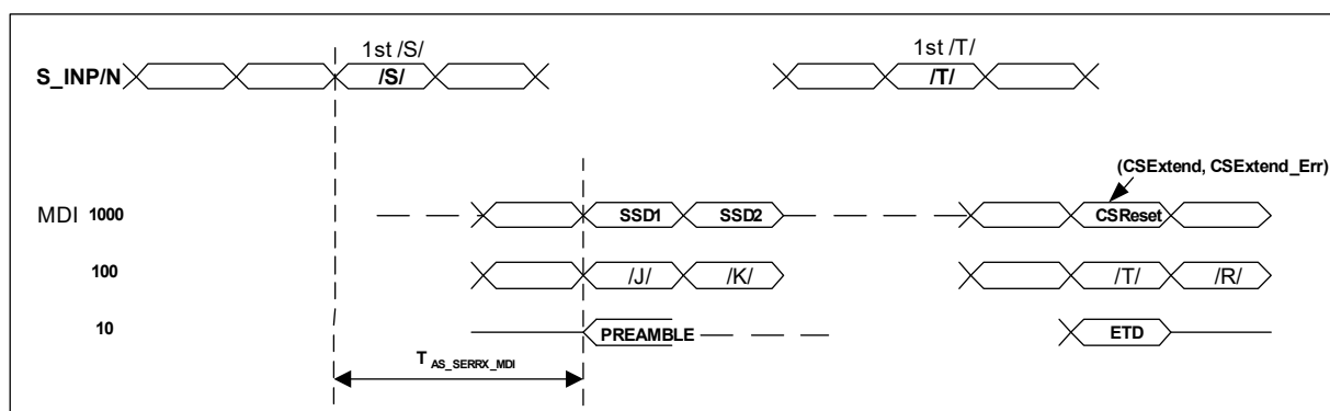
Figure 44: SGMII to 10/100/1000BASE-T Latency Timing
