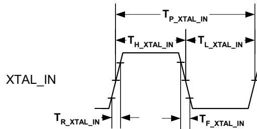
Figure 31: XTAL_IN/XTAL_OUT Timing
