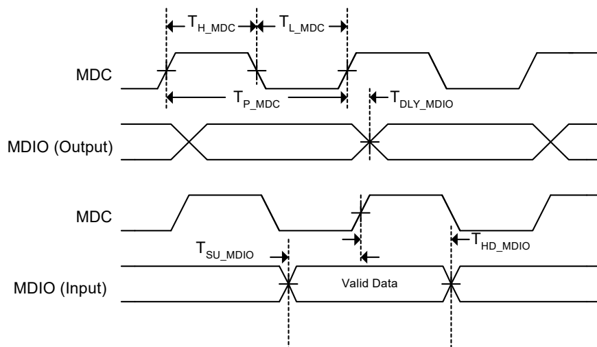
Figure 39: MDC/MDIO Timing
