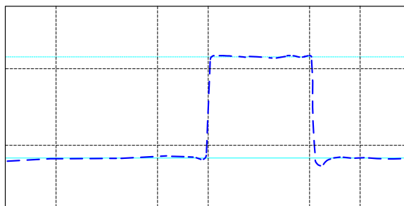
Figure 23: Clean signal after manual calibration for the 60 ohmClean Signal After Manual Calibration for the 60\Omega
