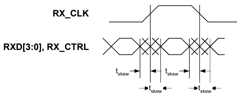
Figure 37: RGMII RX_CLK Delay Timing - Register 21_2.5 = 0
